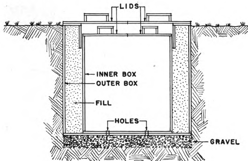
FIGURE 42.—Improvised ice box (double wall).
